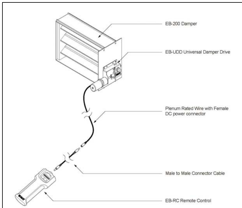
Figure 1 – Illustration for System Connectivity Test
