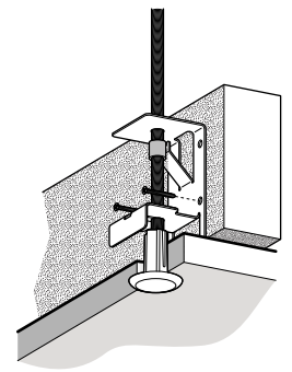
Assembled View
